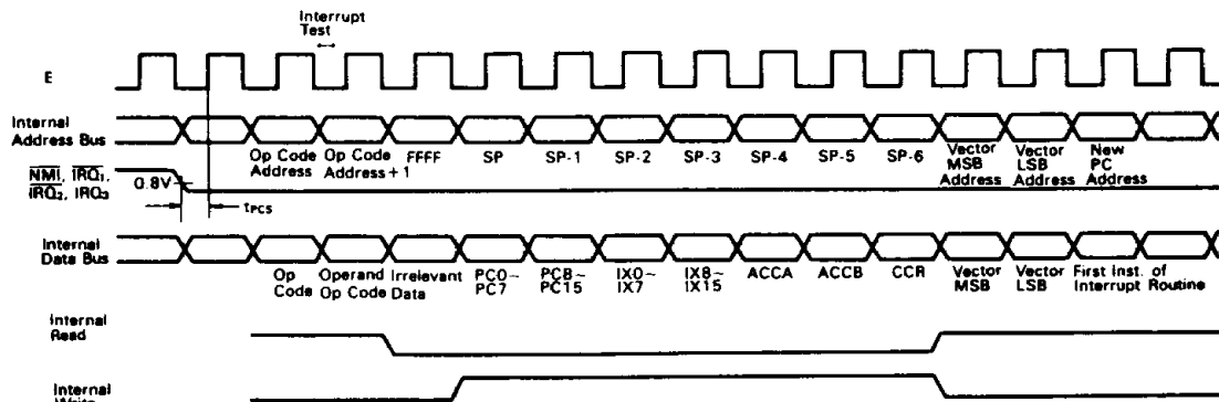
Figure 10 Interrupt Sequence
