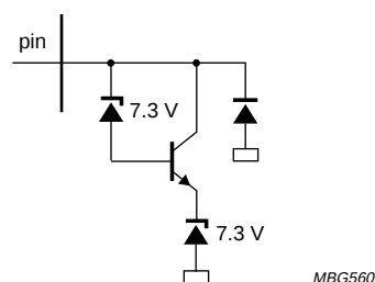
Fig.20 ESD protection for pins 2 to 4, 17 to 24 and 26 to 32.
