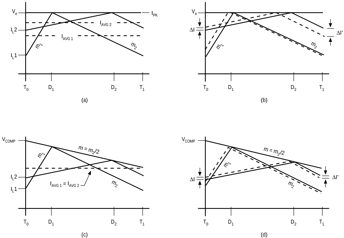
Figure 22. Slope Compensation
