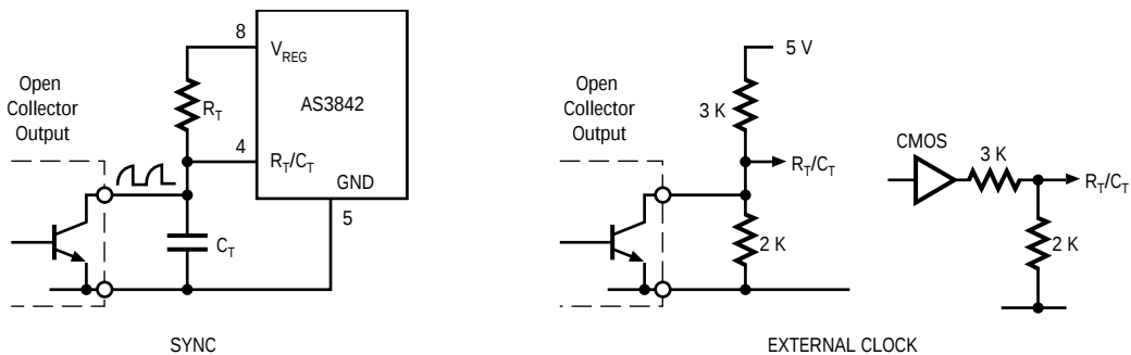
Figure 16. Synchronization
