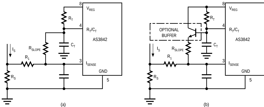
Figure 23. Slope Compensation
