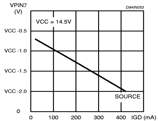
Figure 12. Output Saturation Voltage vs. Source Current
