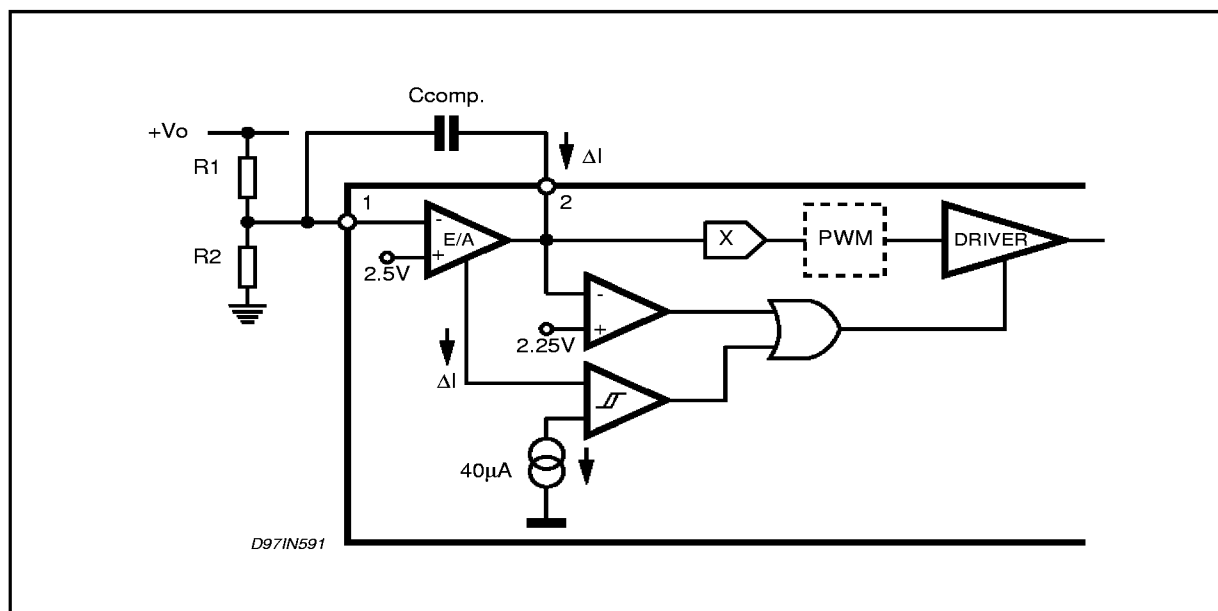
Figure 2. Overvoltage Protection Circuit
