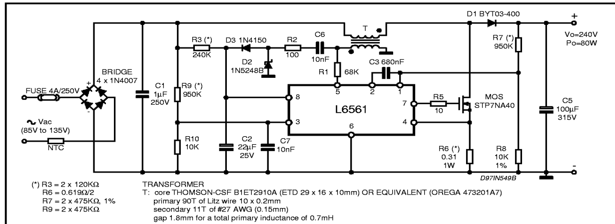
Figure 4. Typical Application Circuit (120W, 220VAC)
