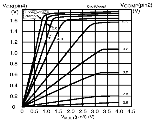
Figure 13. Multiplier Characteristics Family
