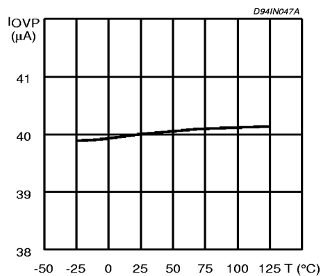
Figure 7. OVP Current Threshold vs. Temperature
