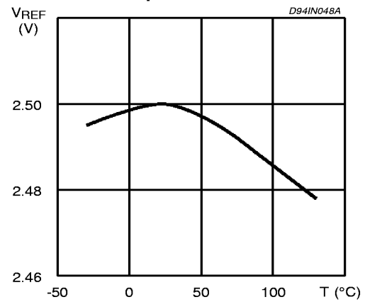
Figure 10. Voltage Feedback Input Threshold vs. Temperature
