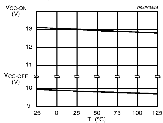
Figure 8. Undervoltage Lockout Threshold vs. Temperature
