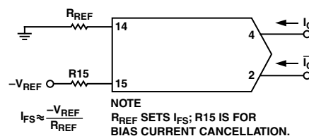
Figure 12. Basic Negative Reference Operation
